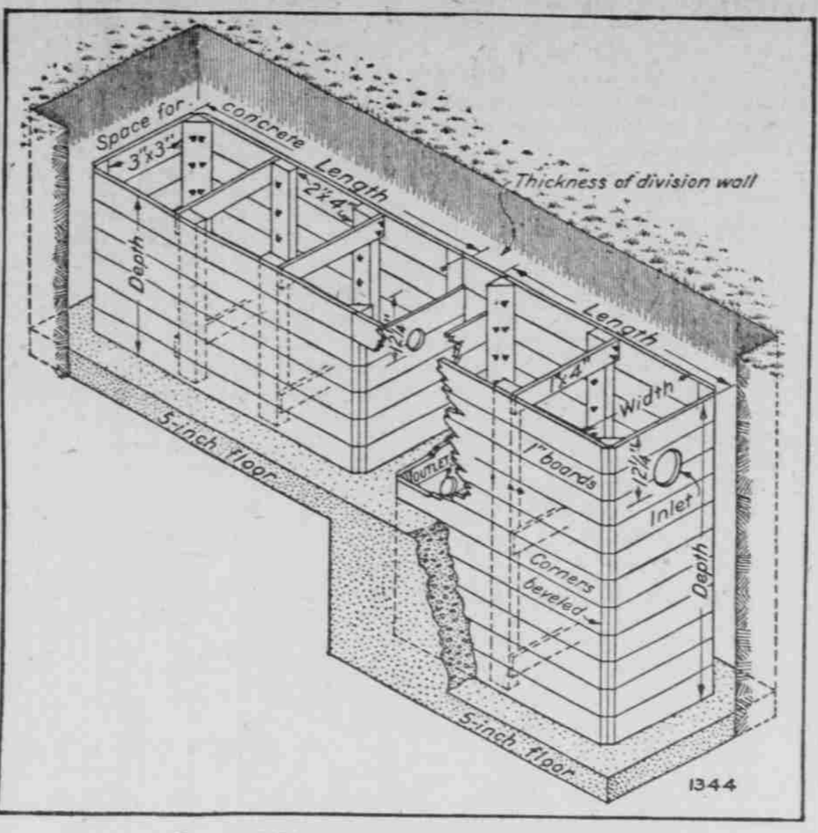
Practical Dimensions for Farm Septic Tank.
