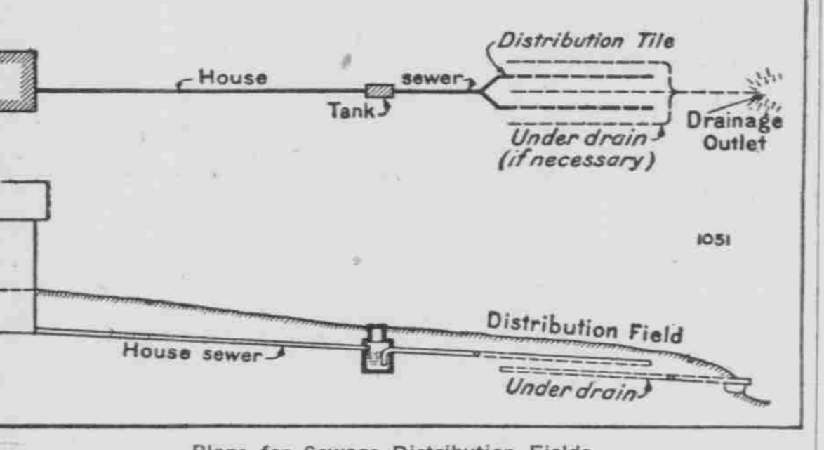
Plans for Sewage Distribution Fields.
