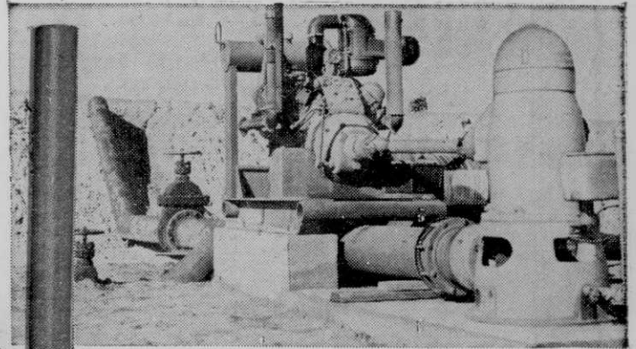
New UV-549 V-8 pumps 1,850 gpm on 10-in. well from 224-ft. level at the Connalt Bros. Ranch, Floresville, Texas.
