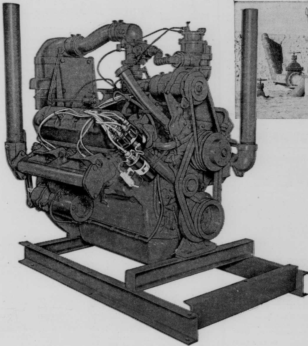
New UV-549 V-8 pumps 1,850 gpm on 10-in. well from 224-ft. level at the Connalt Bros. Ranch, Floresville, Texas.
