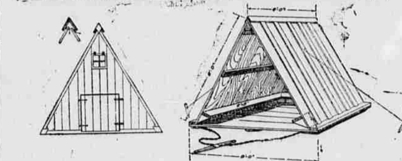
Plan of A-Shaped Hog House; Closed Front on Left. Provision for Ventilation Shown in Small Diagram.
