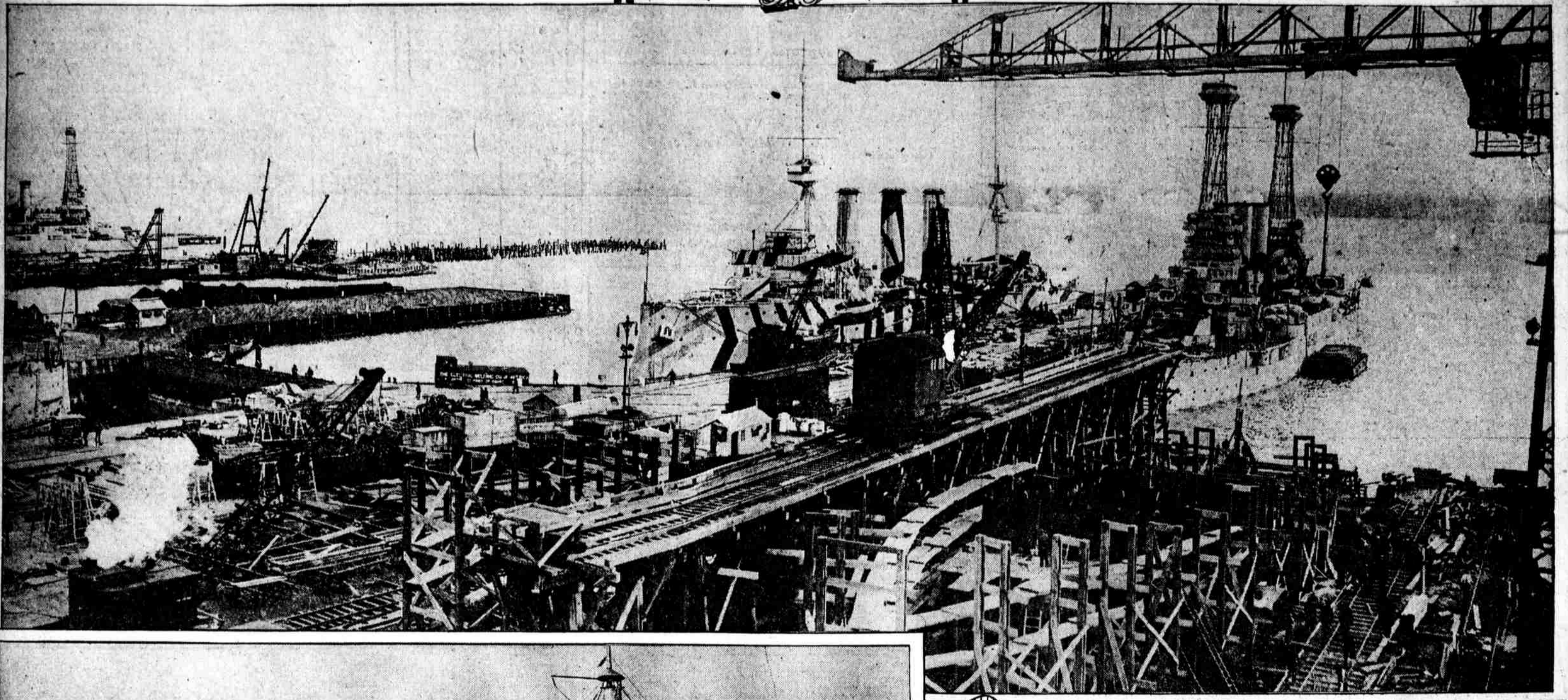
VIEW OF PART OF YARD'S WATERFRONT. In foreground is shipway with vessel in first stages of construction. In center is H. M. S. Cumberland; at right is American battleship.
