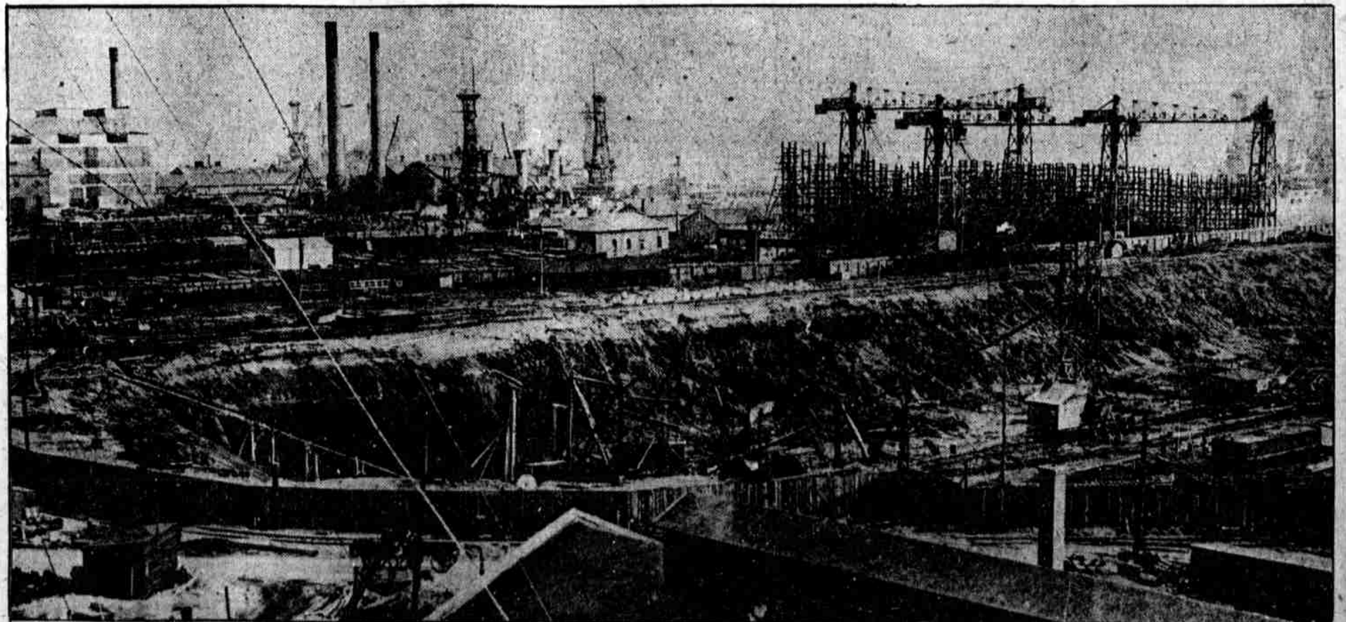
A SECTION OF THE NEW MAMMOTH DRYDOCK under construction. In the distance is a shipway
