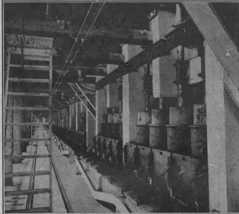
View of one-half or 156 stamps in the Boston Consolidated Mill, Garfield, Utah, installed after a comparative test with Chili Mills, Rolls and the old type 5-Stamp Battery, POSITIVELY PROVING the Nissen Stamp will deliver a more granular and non-silice product than any other mill.
