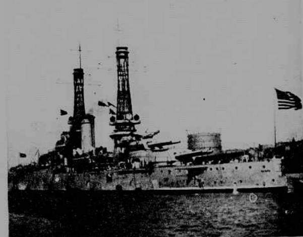
The Battleship NEVADA. Tribune Photo
