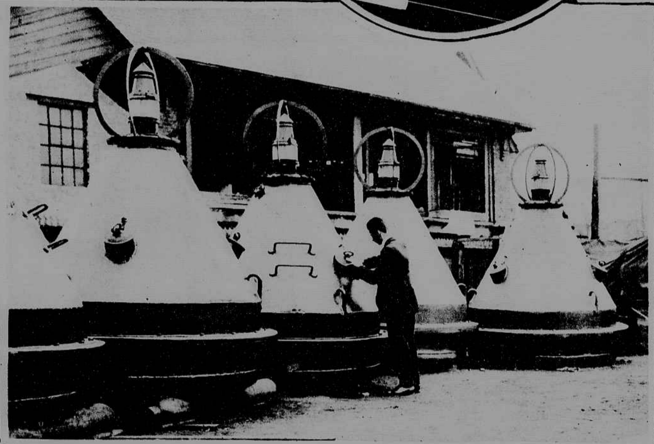
SILENT SENTINELS —automatic shallow water warning buoys that flash unattended day and night for twelve months. By means of a clever storage system sufficient gas to last for a year is stored in these conical structures. A sun valve that is extremely sensitive to light automatically lights the beacons at day-break and extinguishes them at sunset. Underwood
