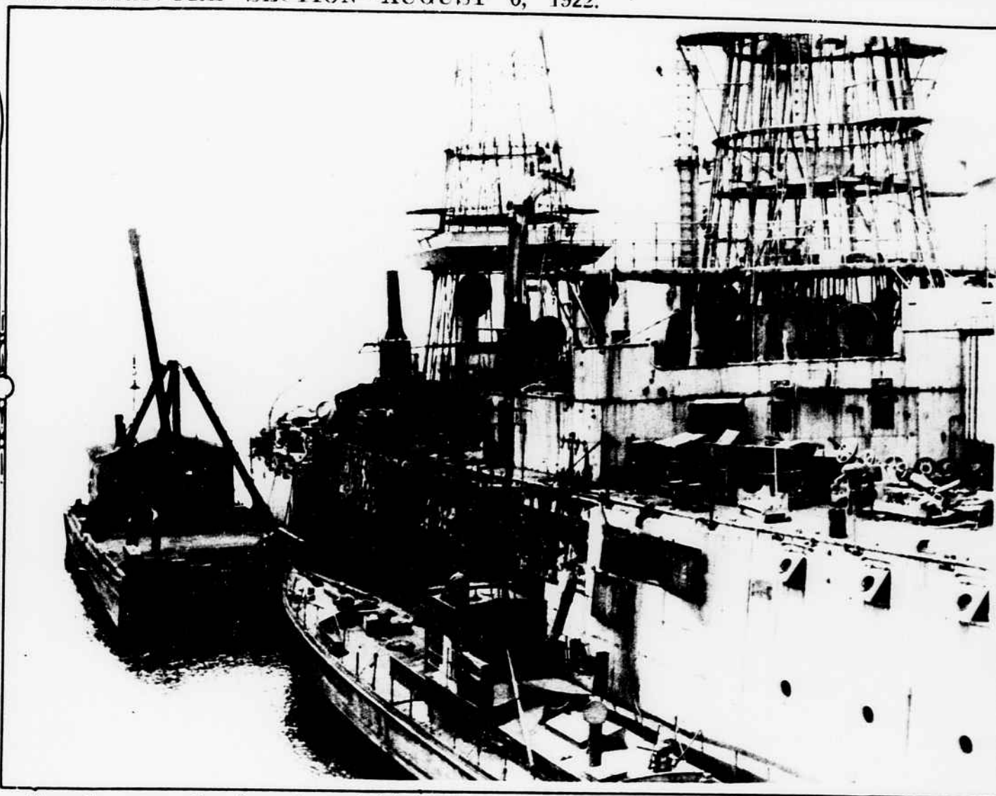
Removing armor plate from the battleship Wisconsin, one of the scrapping processes. This great ship was included in the 845,000 tons of Navy armament to be placed in discard. ©P. & A. Photos
